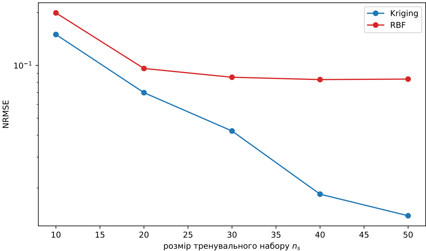
RBF vs Kriging на RD-2D / J (LHS-дизайн)
